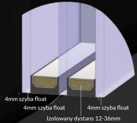
4mm Float + 4mm Float + 4mm Float
