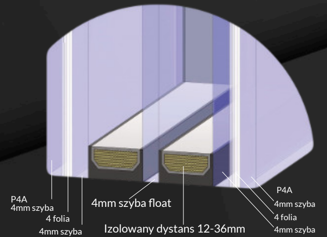
P4A + 4mm Float + P4A
